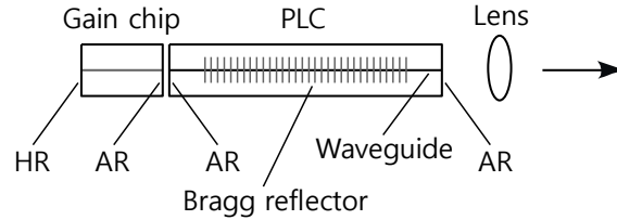
Fig. 1. Schematic of the PW-ECL [11]. HR: high-reflective coating, AR: anti-reflective coating, PLC: planar lightwave circuit. The output is PM fiber-coupled within the butterfly package after the lens and an optical isolator.
