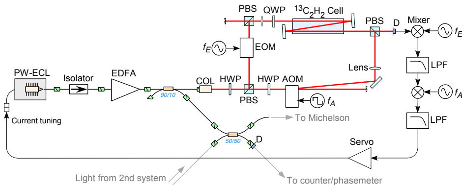
Fig. 4. Frequency stabilization setup using acetylene ( ^{13}\text{C}_2\text{H}_2 ). EDFA: Erbium-doped fiber amplifier, COL: fiber collimator, HWP: half waveplate, QWP: quarter waveplate, AOM: acousto-optic modulator, EOM: electro-optic modulator, PBS: polarized beamsplitter, D: photo-detector, LPF: low-pass filter, f_E : EOM modulation frequency ( \sim 20 MHz), f_A : AOM modulation frequency ( \sim 3 kHz).
