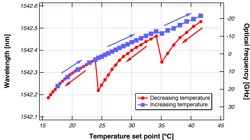
Fig. 2. Frequency (wavelength) tuning by temperature adjustment. Right axis represents optical frequency difference from 1542.383 nm. Circled and squared markers represent tuning results with decreasing and increasing set temperature, respectively.
