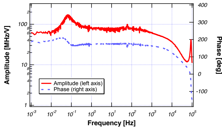
Fig. 3. Frequency tuning transfer function of the PW-ECL through injection current tuning terminal.
